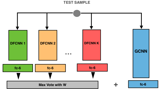
Figure 4. Feature representation of the test image is the concatenated features from both DFCNN with weighting factors and GCNN.
