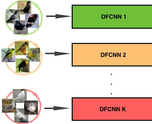
Figure 2. Pre-clustered visually similar images are fed into DFCNN_{1\dots K} with backpropagation training to learn discriminative features for each subset.
